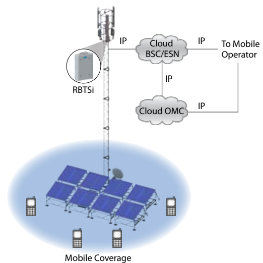
Typical Outdoor 2+2+2 Sector Site (3 RBTSi) with IP radio or VSAT backhaul towards Mobile operator
