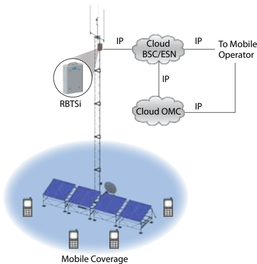
Typical RBTSi Outdoor Omni Site with IP radio or VSAT backhaul towards Mobile operator
