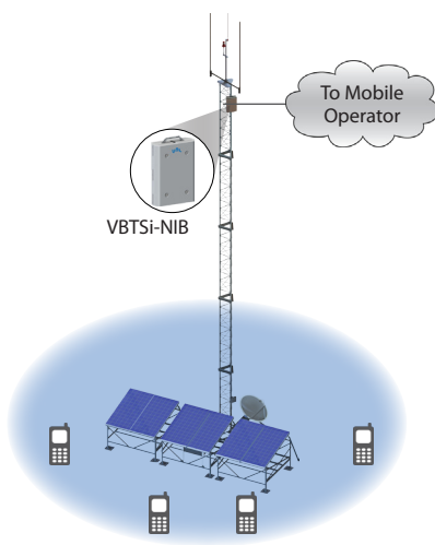
Typical VBTSi-NIB Outdoor Omni Site with IP radio or VSAT backhaul towards Mobile operator
