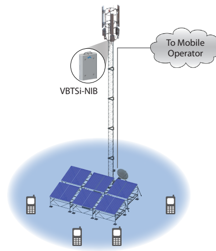
Typical Outdoor 2+2+2 Sector Site (3 VBTSi-NIB) with IP radio or VSAT backhaul towards Mobile operator
